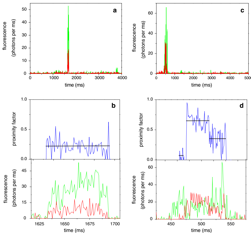
Fig. 3 Photon bursts from double labeled F 0 F 1 QD490–Alexa568 integrated in liposome membranes (excitation at 476 nm). Color code: Donor intensity, FD, QD490 (green), acceptor intensity, FA, Alexa568 (red); proximity factor FA/(FA + FD) (blue). The mean proximity factor is shown as black line. Proteoliposomes are suspended in buffer containing 100 mM MOPSNaOH, pH 7.5, 20 mM succinic acid, 2.5 mM MgCl 2 , 0.6 mM KCl. a photon burst in the absence of ATP, b photon burst from a with expanded time scale and calculated proximity factor, c photon burst in the presence of ATP, d photon burst from c with expanded time scale and calculated proximity factor
