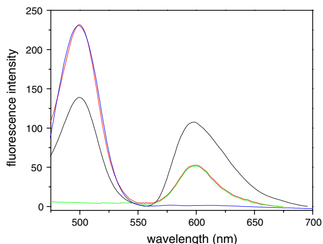
Fig. 2 Fluorescence emission spectrum of F 0 F 1 QD490–Alexa568 (black) and a mixture of QD490 (0.9 \mu M) and Alexa568 (0.5 \mu M) (red). For comparison the fluorescence spectra of the pure QD490 (blue) and pure Alexa568 (green) are shown. Measurements are carried out in 100 mM MOPS–NaOH, pH 7.5
